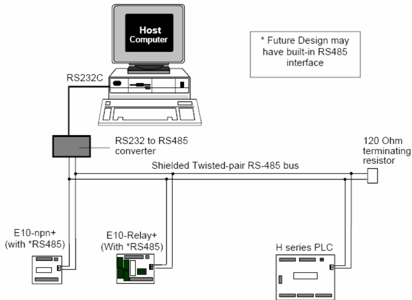
Figure 2-3 - A Multi-drop RS485 network
