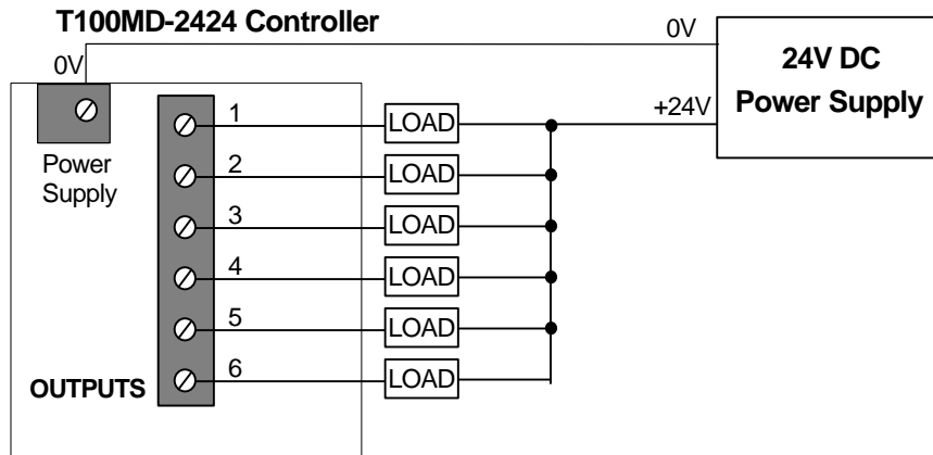
Figure 4 - Transistor Output Interfacing to Load
