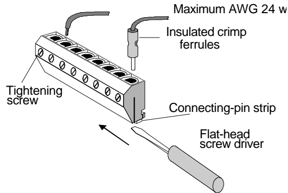
Figure 2 - Removing Screw Terminal block
