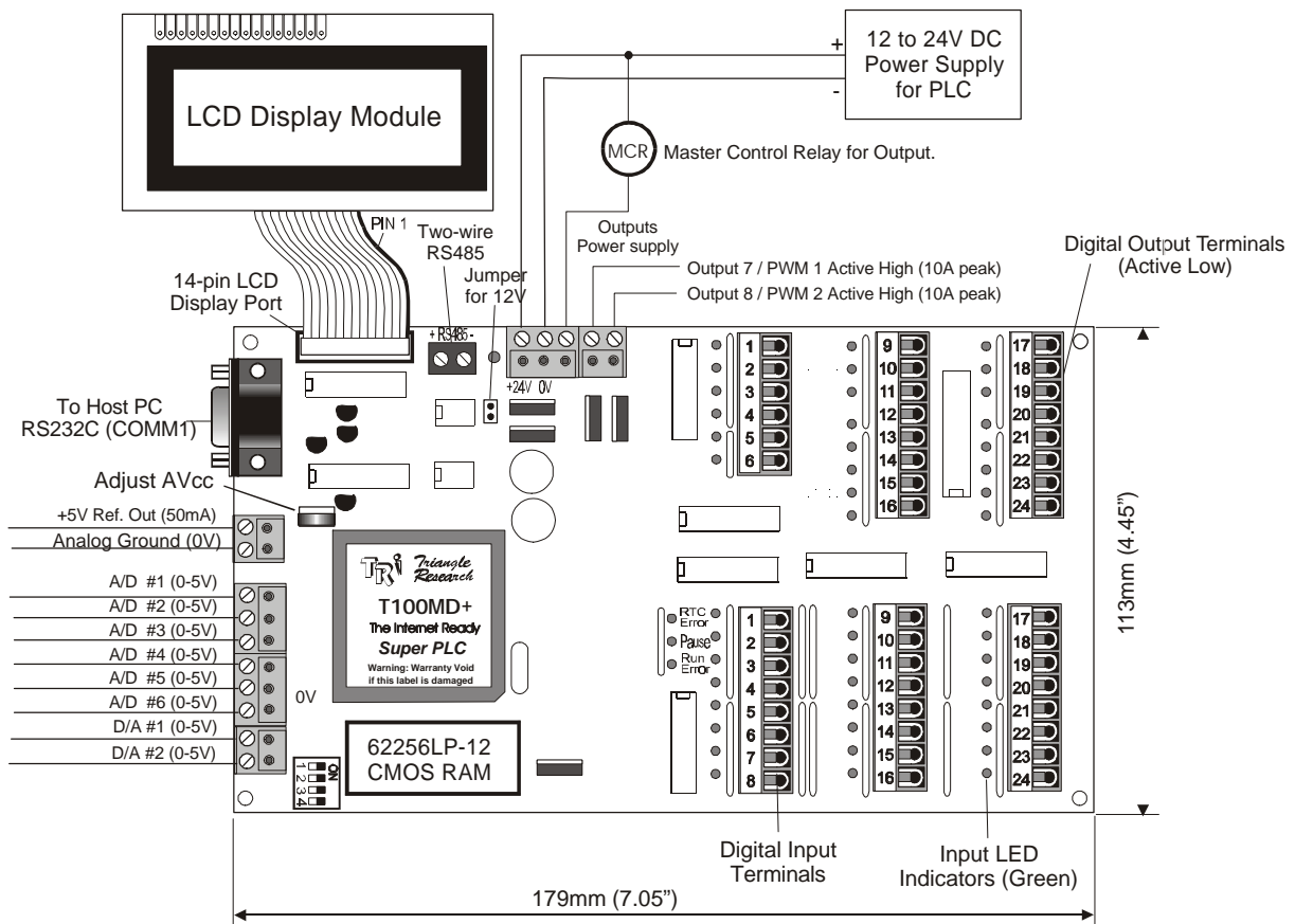
Figure 1 - T100MD-2424+ and a LCD Module
