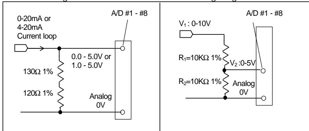
Converting 20mA current-loop to 0-5V
