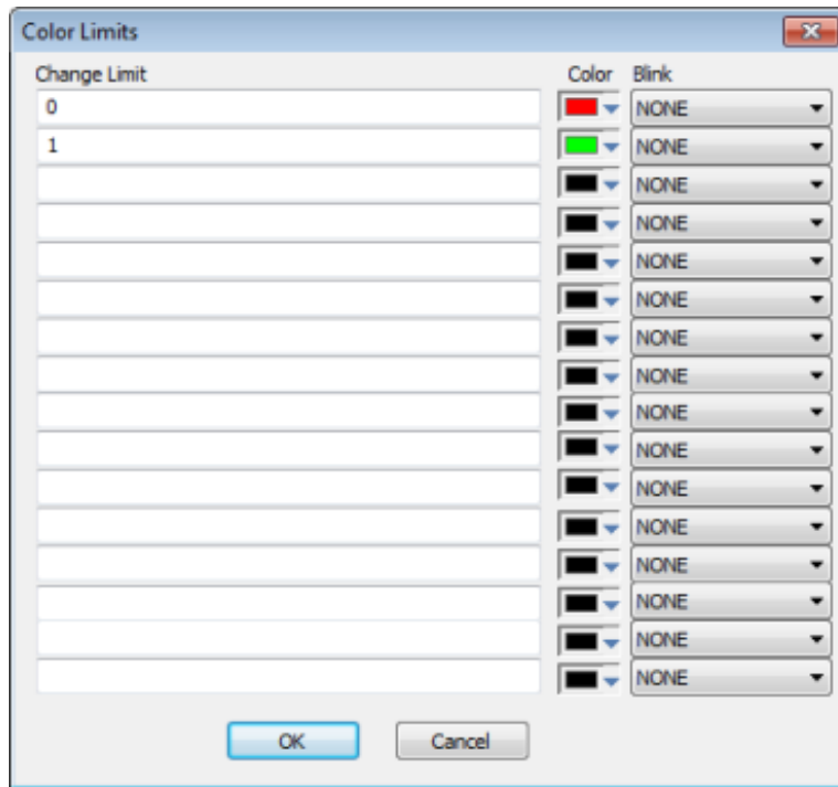
Figure 2. Color Limits dialog
