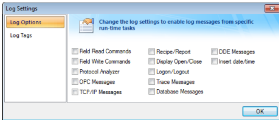
Figure 2. Log Settings — Options Tab
