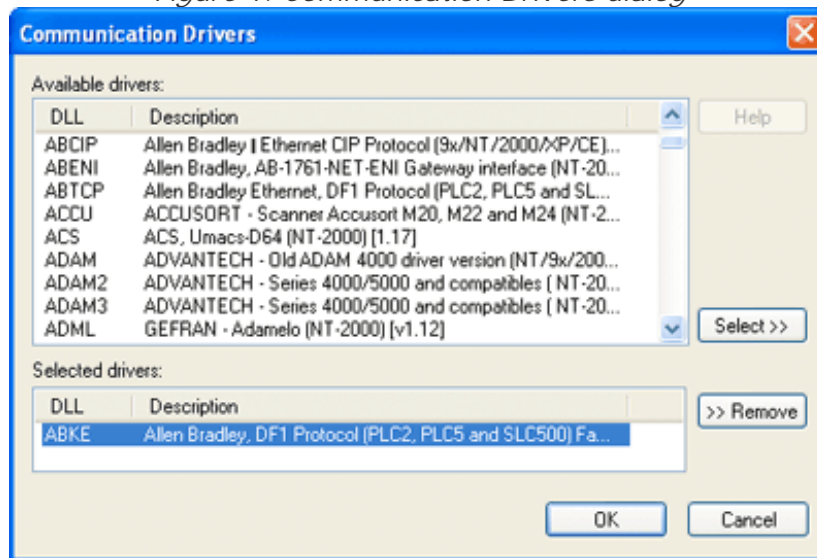
Figure 1. Communication Drivers dialog
