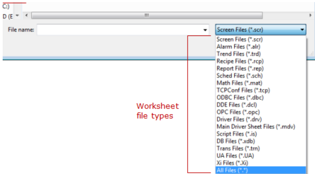
Figure 1. Available worksheet file types in the Open dialog
