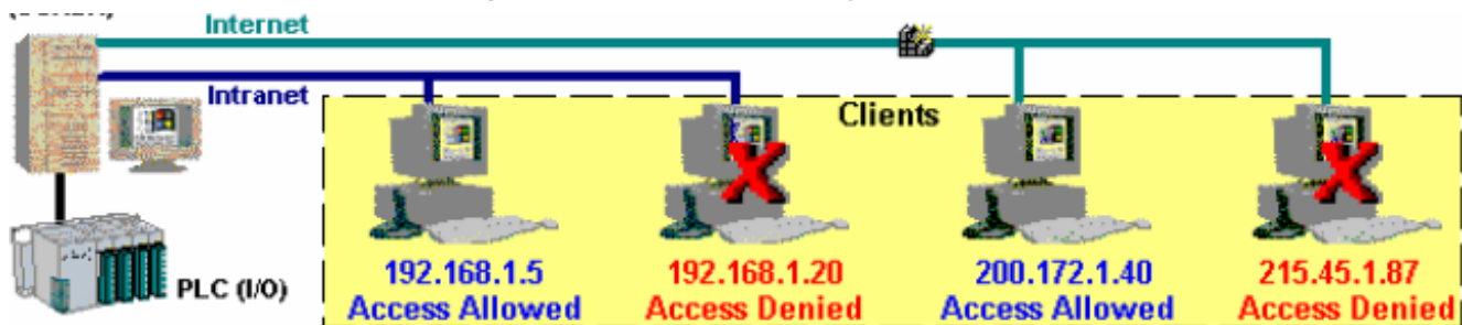
Figure 6. Access allowed by IP address
