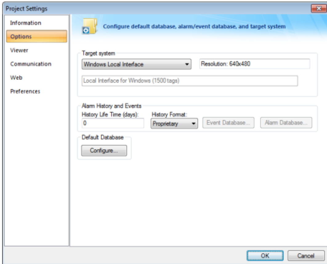
Figure 1. Project Settings: Options tab
