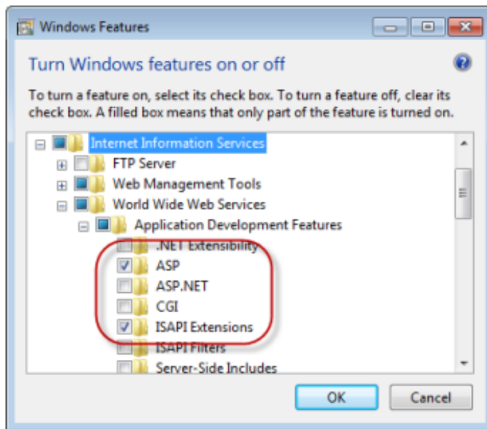
Figure 2. Turning on ASP and ISAPI Extensions in the Windows Features dialog
