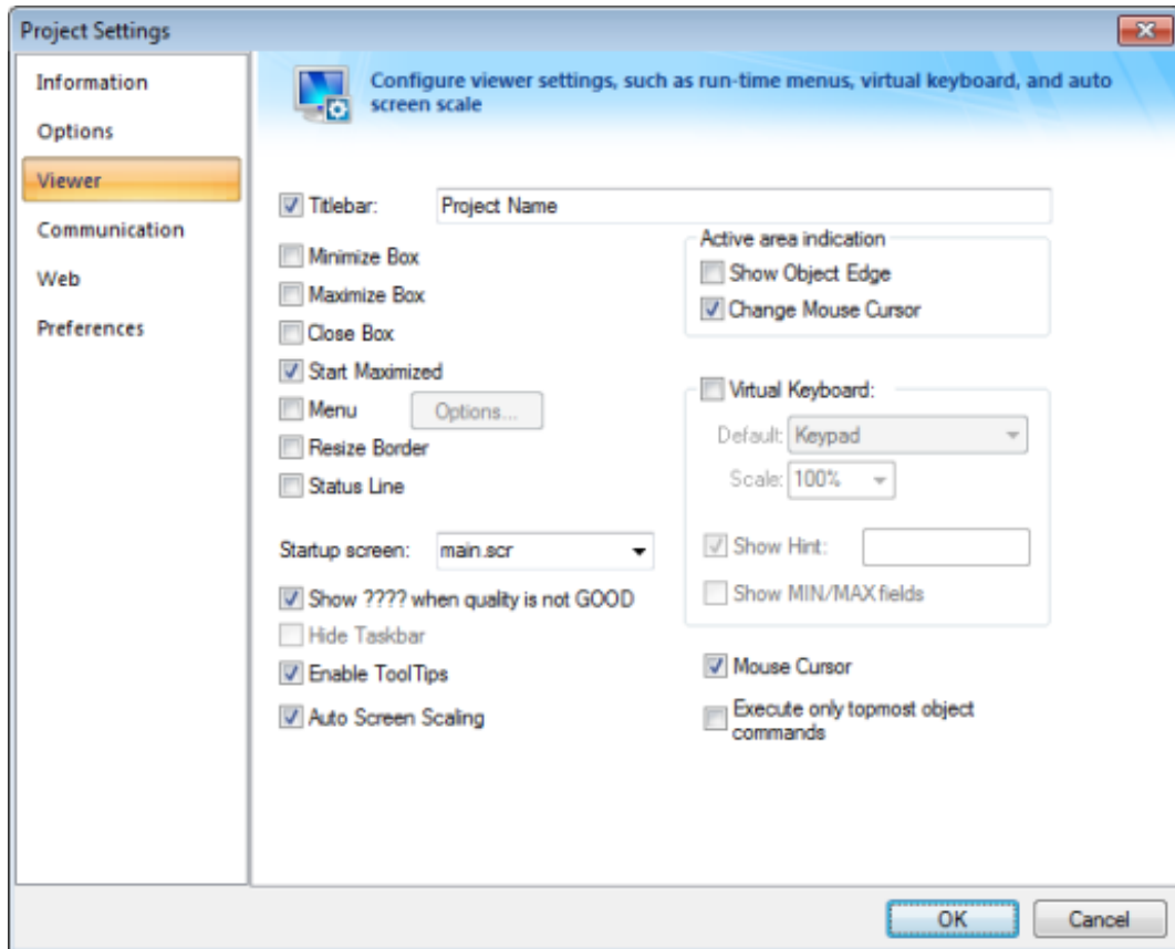
Figure 1. Project Settings: Runtime Desktop tab
