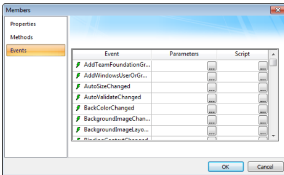
Figure 5. Members Dialog – Events tab
