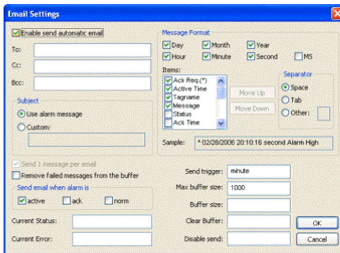
Figure 1. Alarms Worksheet — Email Settings
