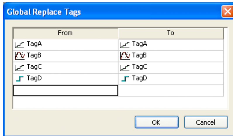
Figure 1. Global Replace dialog
