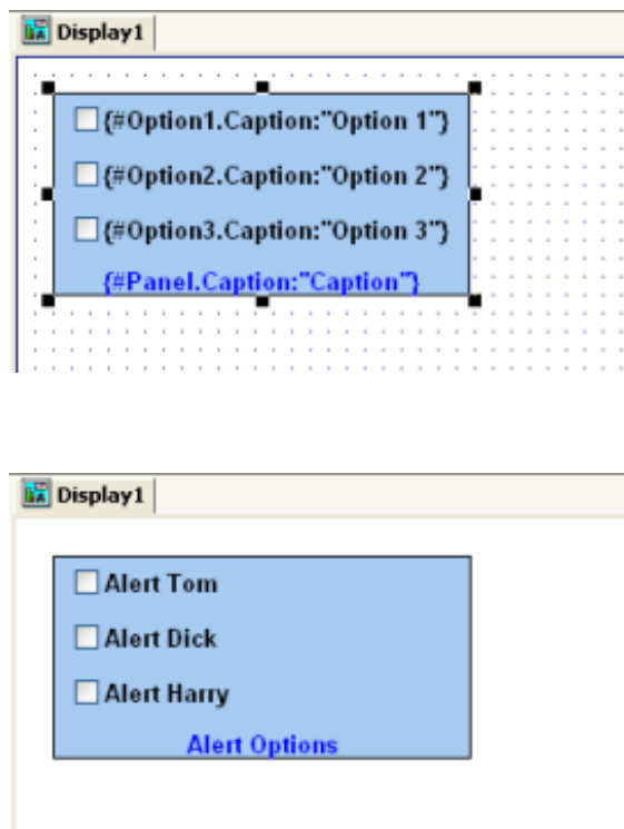
Figure 24. Symbol During Editing (top) and During Runtime (bottom)
