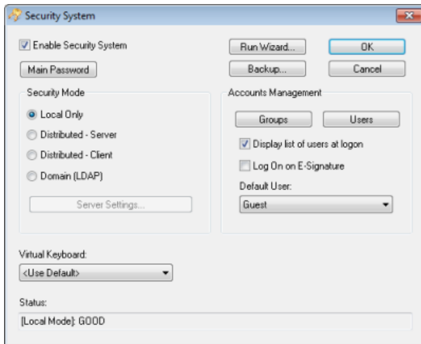
Figure 1. Security System dialog
