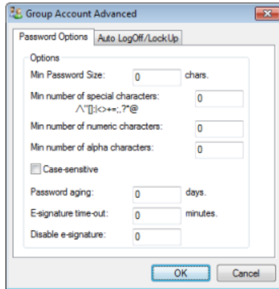
Figure 2. Advanced dialog – Password Options
