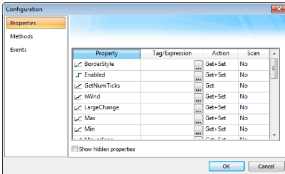
Figure 3. Configuration Dialog – Properties Tab
