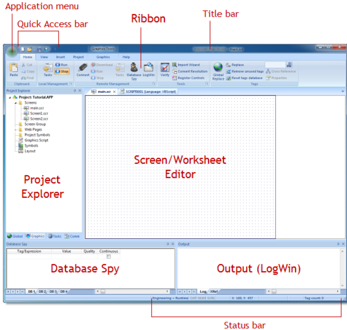
Figure 1. The IWS Development Environment
