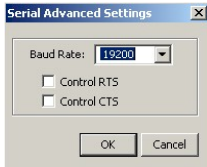
Figure 3. Serial Advanced Settings dialog
