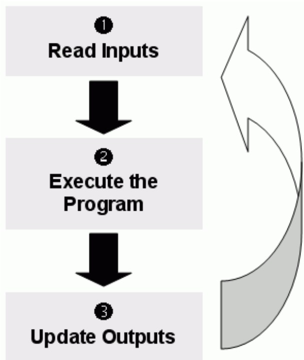
Figure 1. PLC Program Loop
