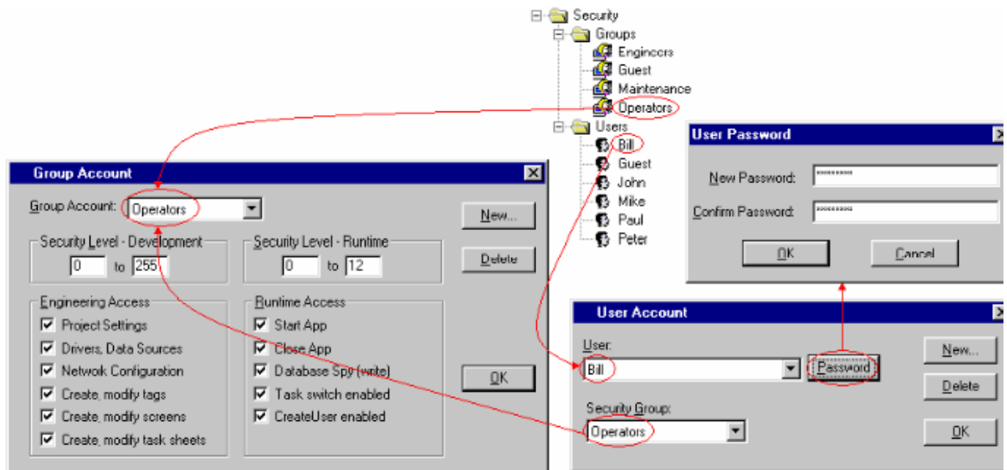
Figure 1. Security Groups and Users
