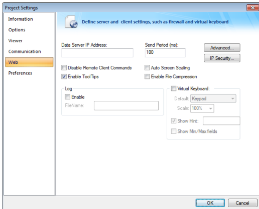
Figure 1. Project Settings dialog — Web tab
