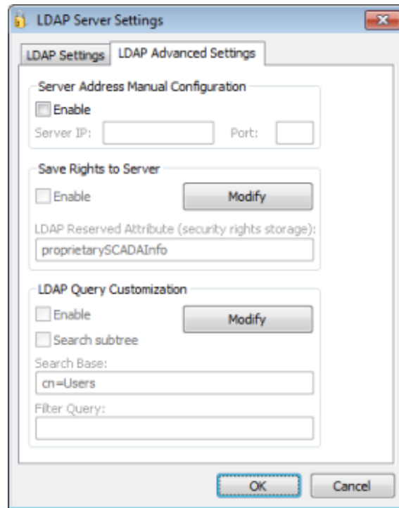
Figure 3. LDAP Advanced Settings
