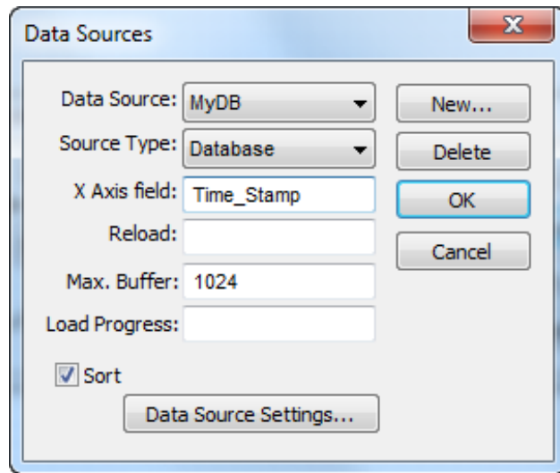
Figure 3. Setting X Axis field to Time_Stamp
