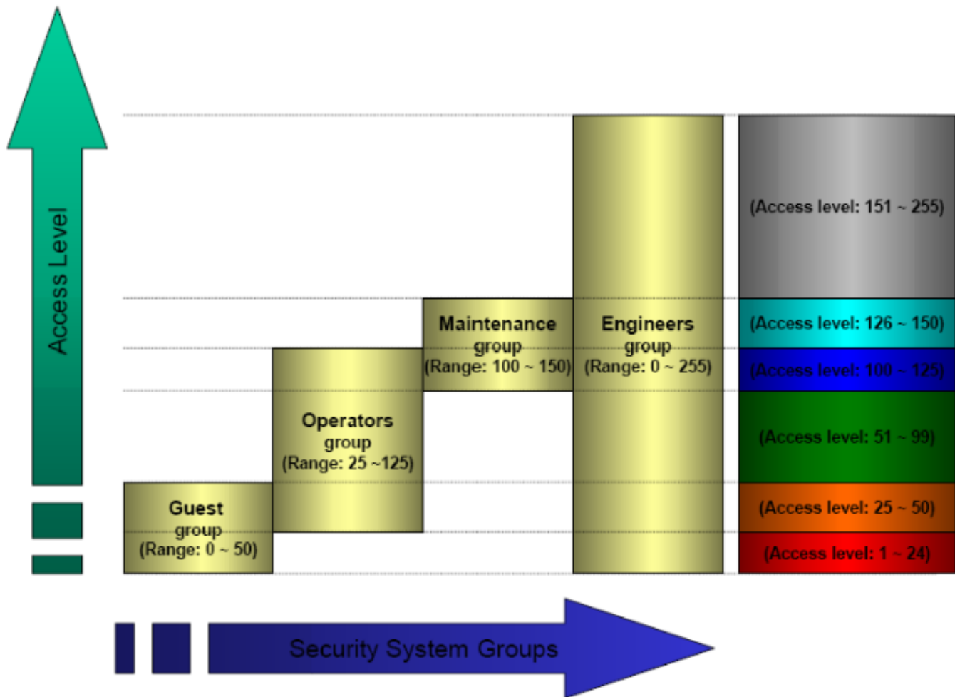
Figure 1. Example of security access levels
