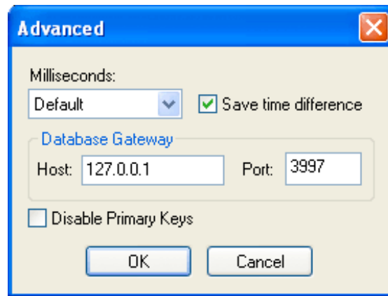
Figure 3. Database Configuration: Advanced dialog
