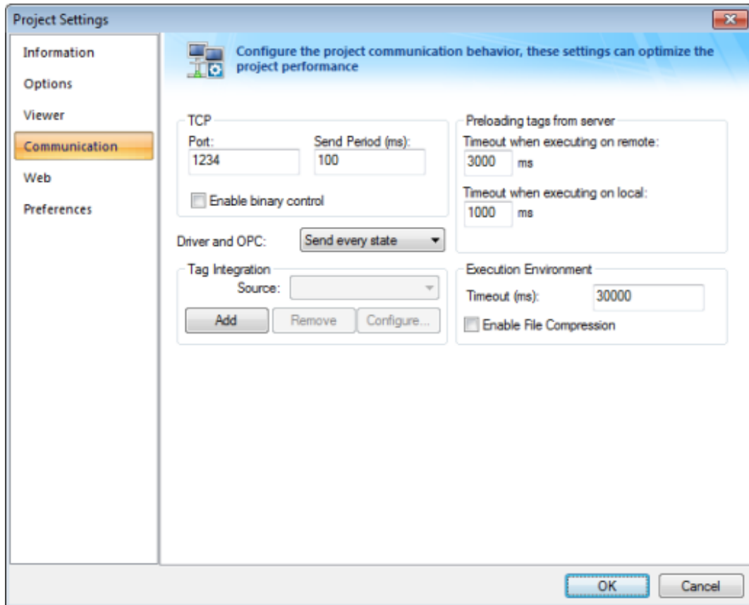
Figure 1. Project Settings: Communication tab
